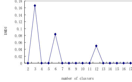
Fig. 8. Differential MDI curve of lenses at Min-support=0.8
