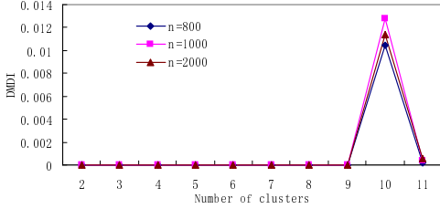
Fig. 35. Sample DMDI curves of T20I500D20K-N1000 at Min-support=0.8
