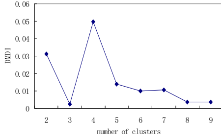
Fig. 19. DMDI curve of soybean-small at Min-support=0.8
