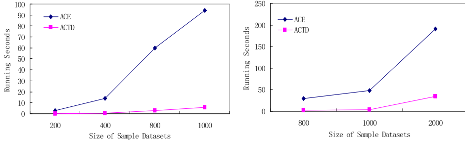
Fig. 31. Running time of ACTD Fig. 32. Running time of ACTD and ACE on T50I1000D1K Sample and ACE on T20I500D20K Sample datasets
