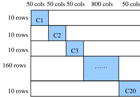
Fig. 11. Structure of one layer synthetic data
